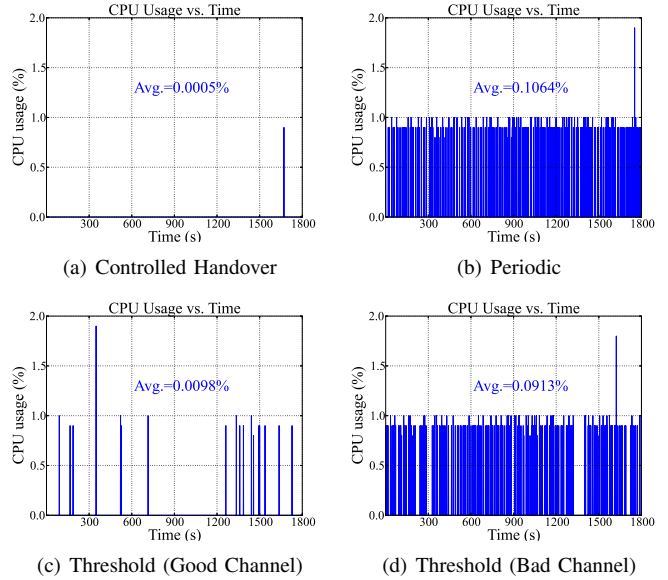
Fig. 5. CPU loading of different triggering mechanisms
